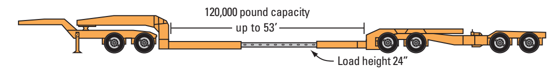
Multiple Axle High Tonnage Double Drop
