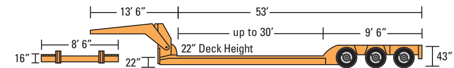
Removeable Gooseneck
