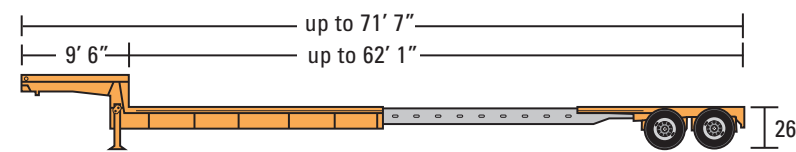
Extendable Single Drop
