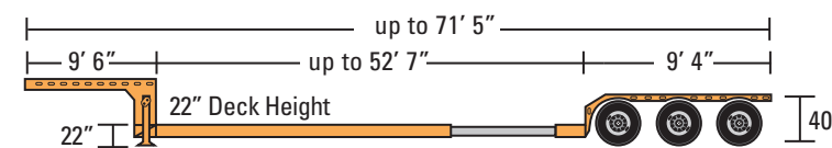
Extendable Three Axle Double Drop
