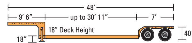
Double Drop
